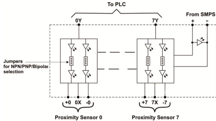
Wiring Diagram
